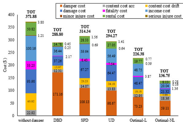
Figure 3. Comparison of cost components for different damper designs and without damper for one square meter in the 7 story structure
