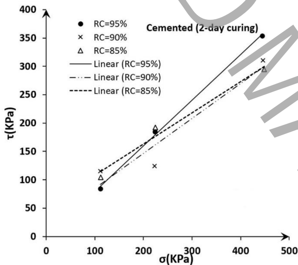
Figure 3. Effect of RC on the strength parameters of cemented carbonate soil of Khark (Curing time=2 days)
