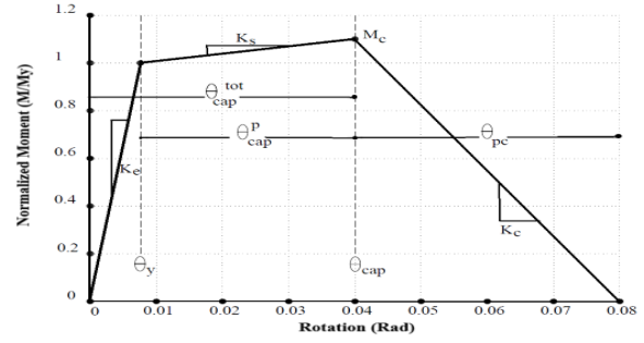
Fig.1 Tri-linear backbone curve of the plastic hinge model
