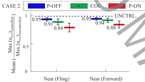
Figure 2. Mean and standard deviation of normalized maximum roof displacement for the 3 rd alternative of the controlled structure (i.e., damper at the fifth floor) under near-fault record sets earthquakes.
