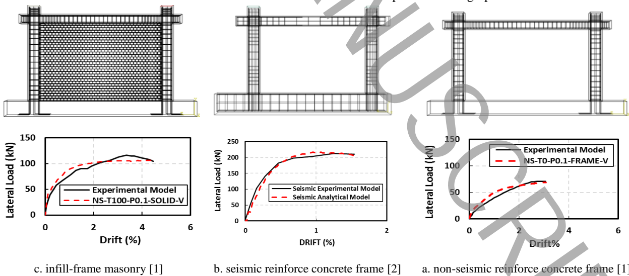
Figure 1. Verification of laboratory model with FE model
