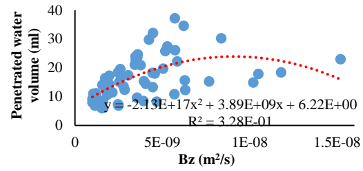
Figure 6. Correlation between optimum \beta_z and penetrated water volume.
