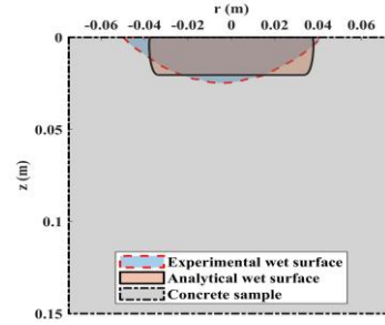
Figure 2. Analytical and experimental wet curves ( W/C = 0.4 , p = 0.95 \text{ MPa} and t = 0.5 \text{ h} ).
