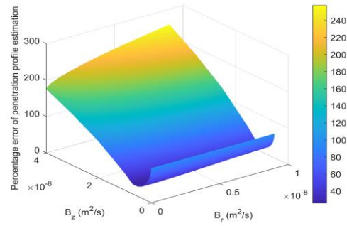
Figure 3. Diffusion coefficients-percentage errors graph ( W/C = 0.5 , p = 0.50 \text{ MPa} and t = 0.5 \text{ h} ).
