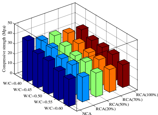
Figure 1. Compressive strength RCA (%) - W/C relationship.
