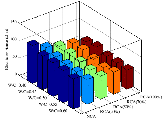
Figure 2. Electric Resistance RCA (%) - W/C relationship (90days).
