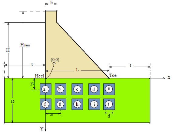
Figure 1: Two-dimensional view of the gravity dam and its foundation in the present study
