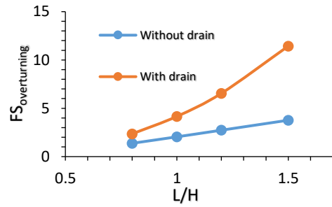
Figure 3: Effect of L/H on safety factor against overturning with and without of drains
