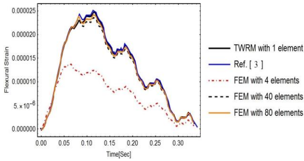
Figure 2 Flexural Strain at x=0.25L
