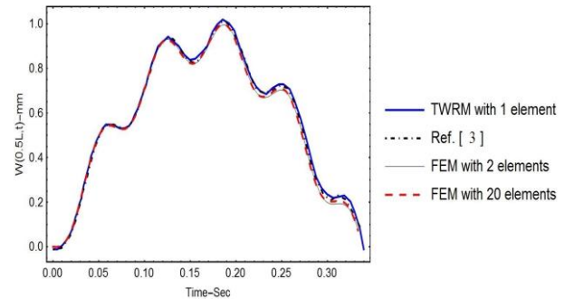
Figure 1 Deflection at x=0.5L
