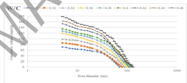
Figure 2. Effect of water to cement ratio on concrete porosity
