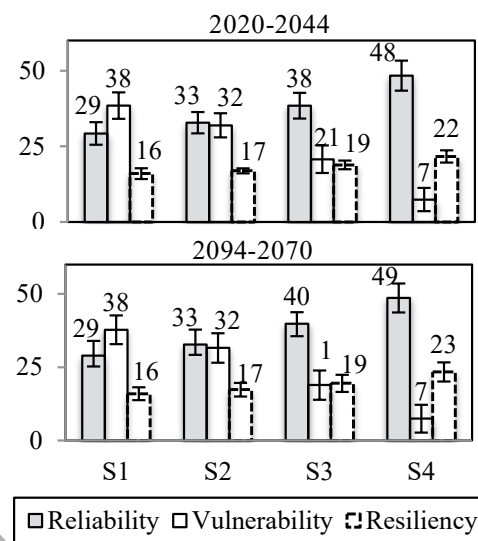
Fig. 2. Reservoir performance indices for different water use efficiency in the future periods
