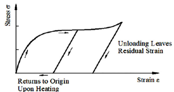
Figure 2. Super-elastic behavior of SMAs [3]
