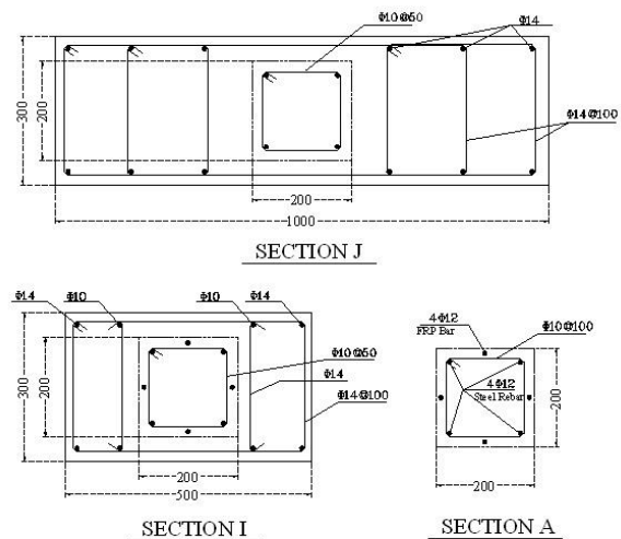
Figure1. Geometry of modeled specimen (dimensions in mm).
