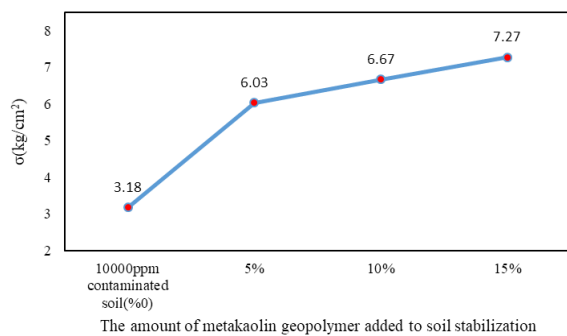
Fig. 2. The changes in maximum UCS of contaminated soil stabilized with metakaolin geopolymer cured in 7 days
