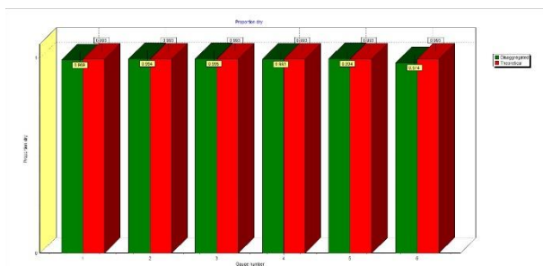
Fig. 1. Comparison of the dry period ratio of observed (used in the model) and simulated hourly rainfall series I
