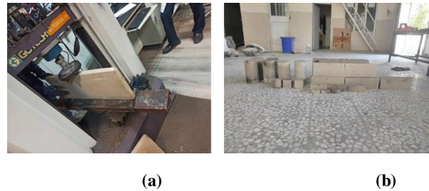
Figure 1- (a) Sample with d=304.8 mm under bending test (b) Samples of mixing design A1
