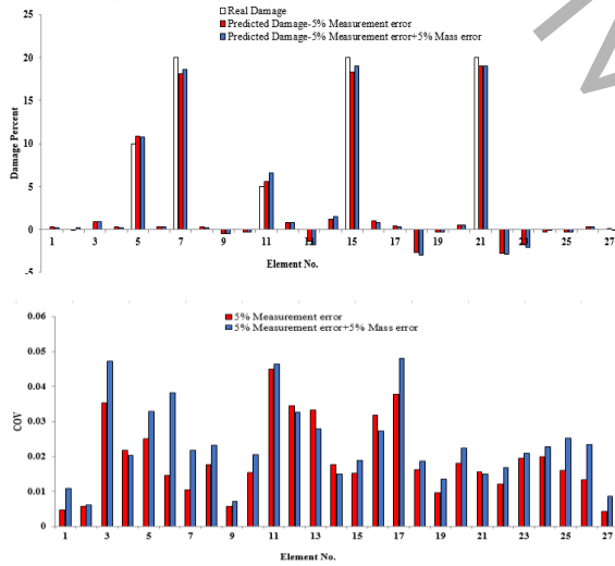
Figure 2. (a) First case damage predicted parameter at considering 5% measurement error and 5% modeling error, b) COV of the predicted parameters.
