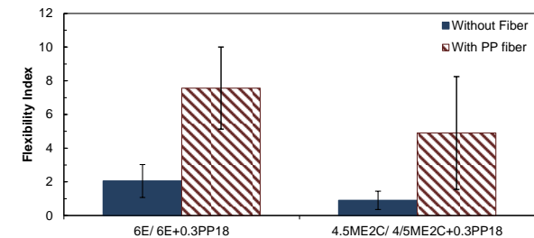
2.c: SCB Flexibility Index results
