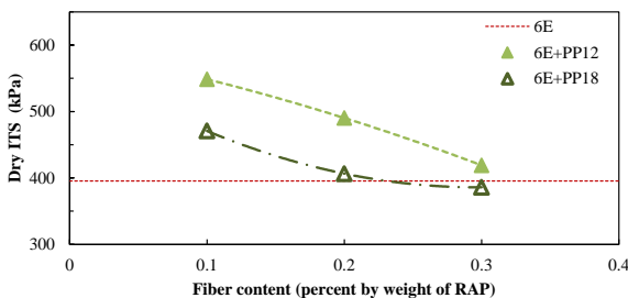
1.a: Dry ITS results
