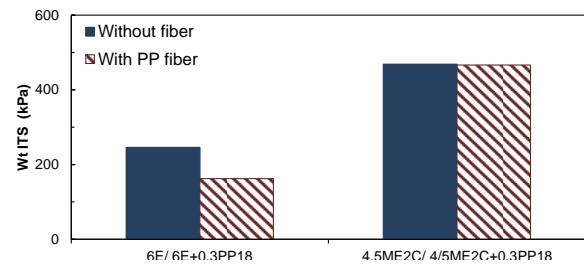
2.b: Wet ITS results
