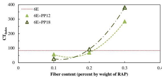
1.c: IDEAL-CT CT_{Index} results
