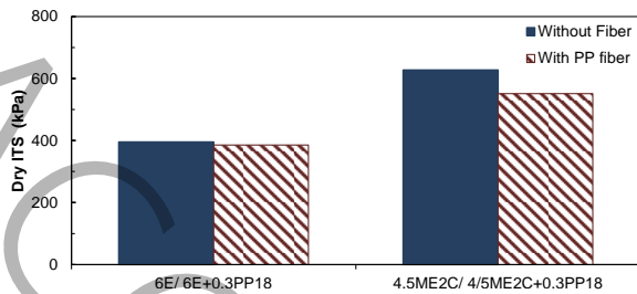
2.a: Dry ITS results
