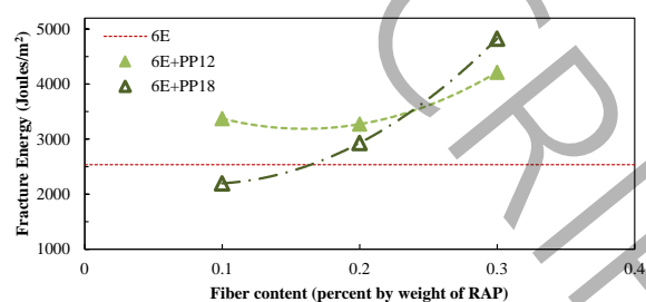
1.d: IDEAL-CT fracture energy results
