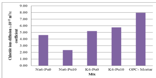
Figure 2: Chloride ions diffusion coefficient ( D_s ) of submerged specimens in Persian Gulf
