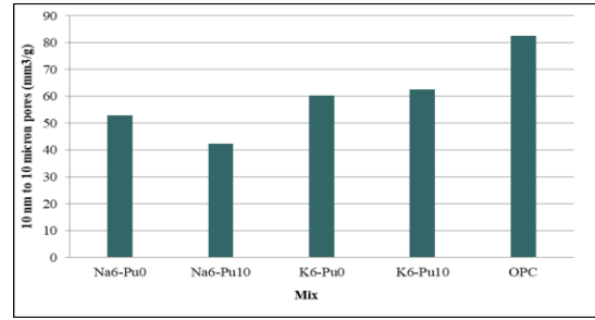
Figure 3: 10 nm to 10 \mu\text{m} pores of mortars
