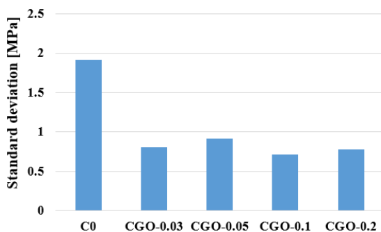
Figure 1. Standard deviation of compressive strength results.
