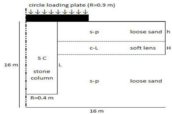
Figure 1. 2D schematic of model properties
