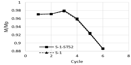
Fig. 4. Comparison of the final strength of S-1.
