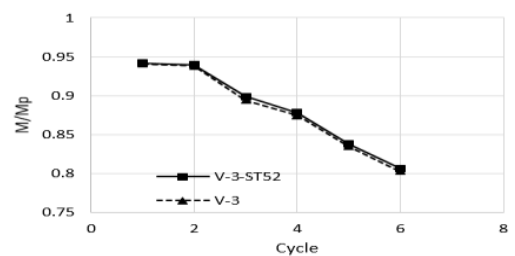
Fig. 6. Comparison of the final strength of V-3.
