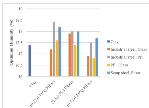
Fig. 4. Graph of optimal humidity of soil combined with fibers in pairs and with different percentages
