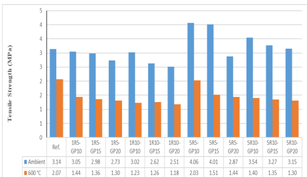
Figure 3. Splitting tensile strength of mixtures at ambient temperature and 600 °C
