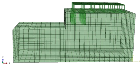
Figure 2-Geometrical view of the concrete structure with excavation and micropiles
