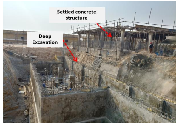
Figure 1. The concrete construction near the excavation has suffered subsidence.
