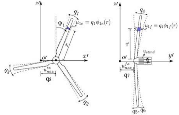
Figure 1. Degrees of freedom [4]
