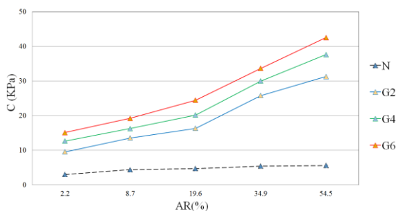
Figure 5: Changes in the cohesion value of the slag-sand column composite
