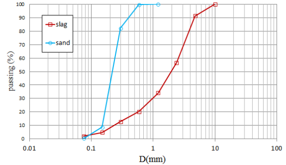
Figure 1: Sand and slag grading curves
