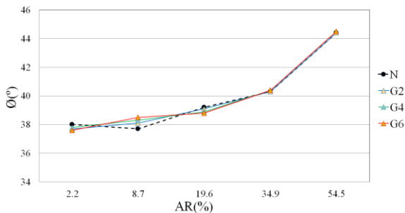
Figure 4: Variations of internal friction angle of slag-sand column composite
