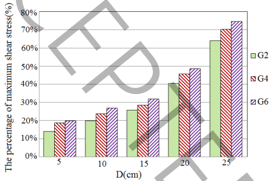
Figure 3: The percentage of the maximum shear stress of group samples compared to the maximum stress of sand
