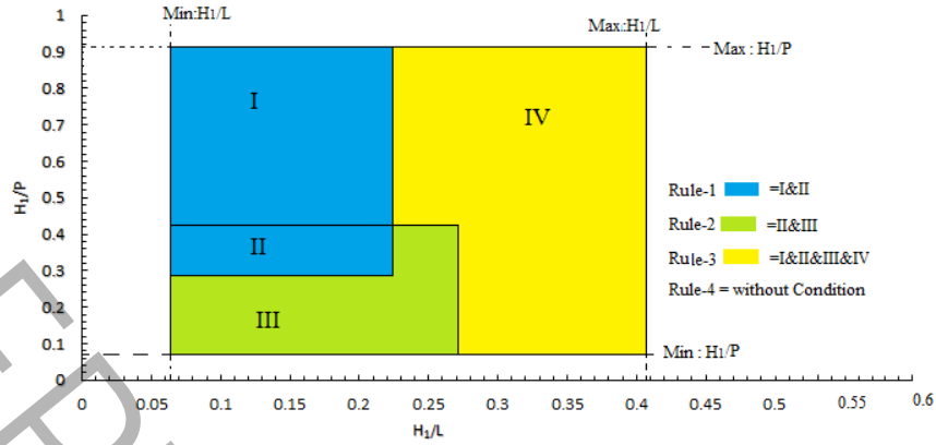
Fig. 2 Specified zones obtained from “If-then” rules
