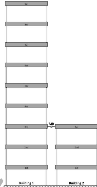
Figure 1. Model of two adjacent buildings [14] connected with MR damper
