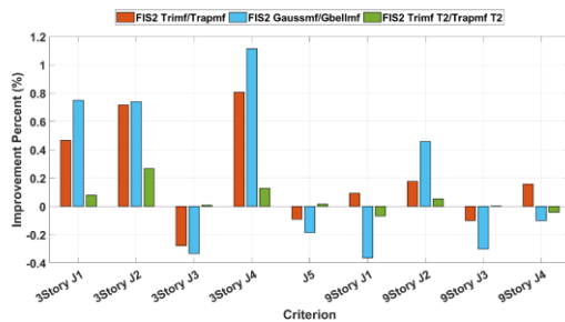
Figure 3. Comparison of type 1 and type 2 FIS2 systems with different membership functions
