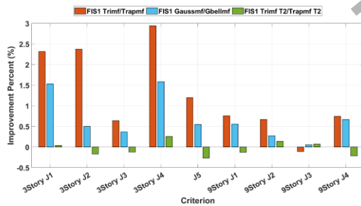
Figure 2. Comparison of type 1 and type 2 FIS1 systems with different membership functions
