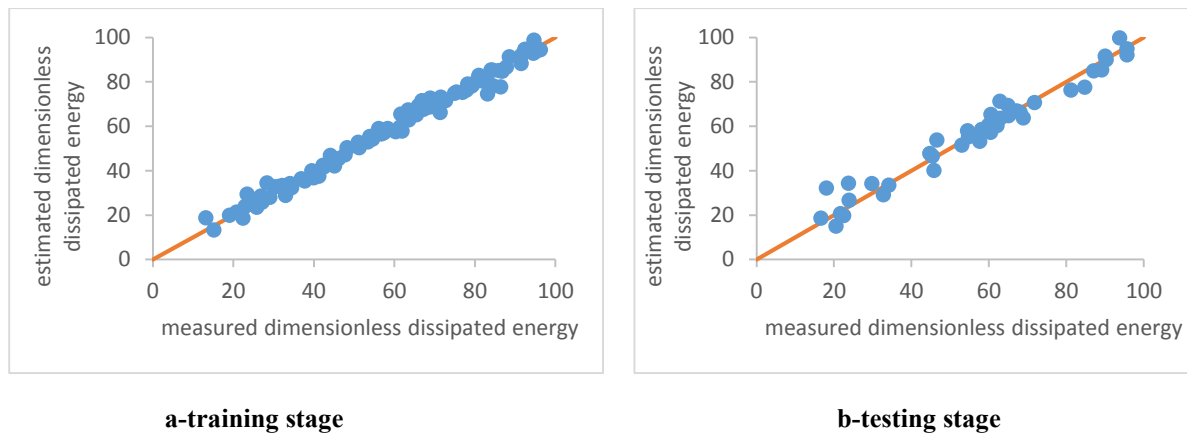
Fig. 1. Results of ANFIS-FA algorithm in the prediction of energy loss with all input parameters
