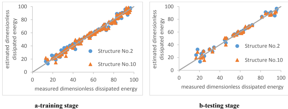
Fig. 2. Results of the best structures of the GEP algorithm for the prediction of dissipated energy with all input parameters.
