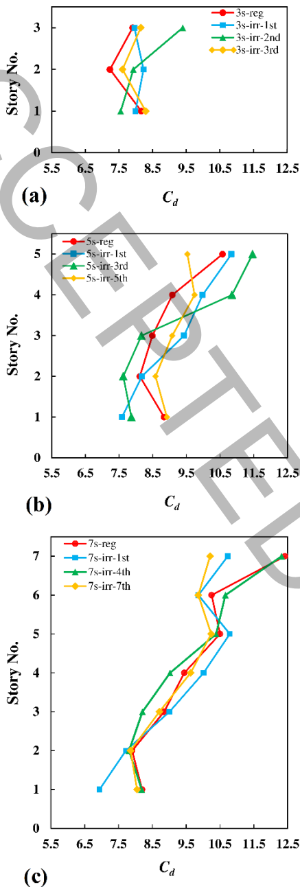
Figure 1. Obtained mean C_d values for the (a) 3-, (b) 5- and (c) 7-story structures
