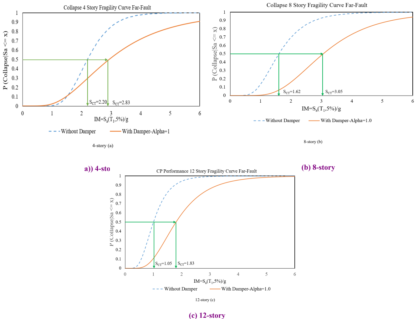
Fig. 2. Comparison of the fragility curves for the buildings studied with and without the viscous damper.
