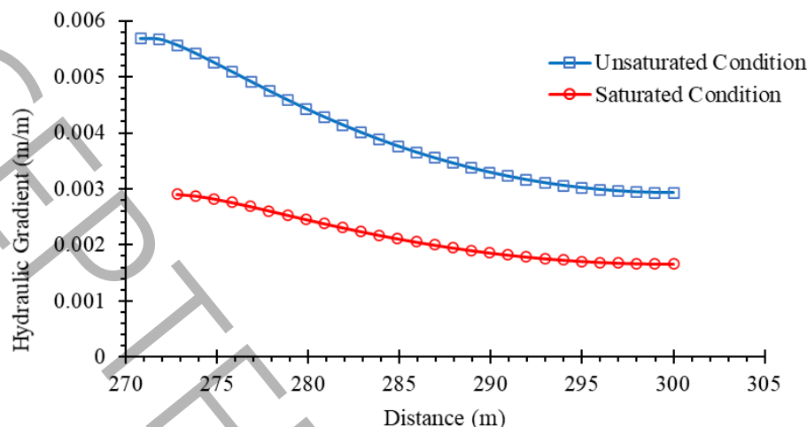
Fig. 12. The changes of the exit hydraulic gradient in the downstream of the embankment dam for two saturated and unsaturated flow conditions
