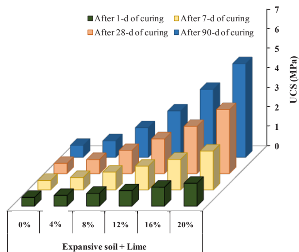
Fig. 1. Effect of lime alone on the UCS of soil sample at different times of curing.
