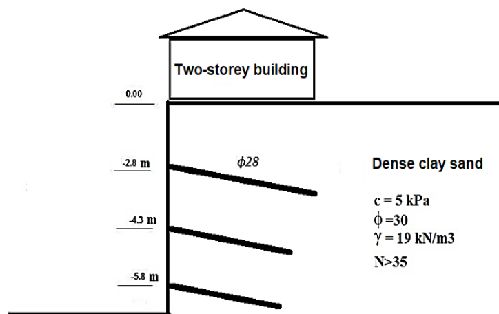
Fig. 1. Section of the nailing of Daroos project
