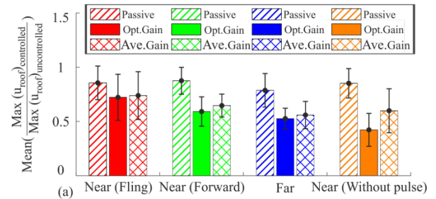
Fig. 4. Comparison of average and standard deviation of structural responses with optimum and average actuator power
