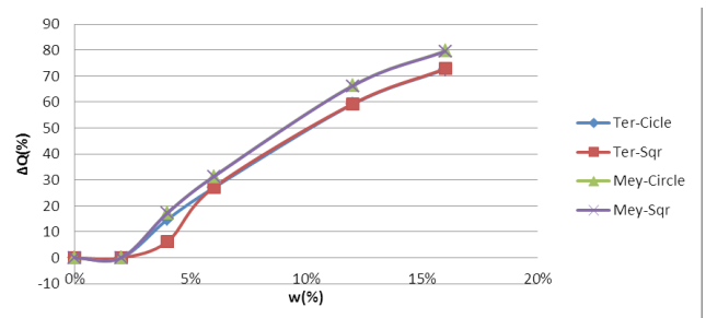
Figure 3. Relative reduction in ultimate bearing capacity in 75% compaction
