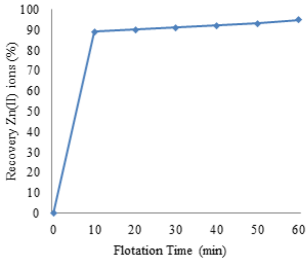
Figure 1. Zn(II) ions recovery as a function of the flotation time. (SDS=300 ppm, Dowfroth 250=90 ppm, Zn(II)=10 ppm, pH=3 and agitating speed=1000rpm)
